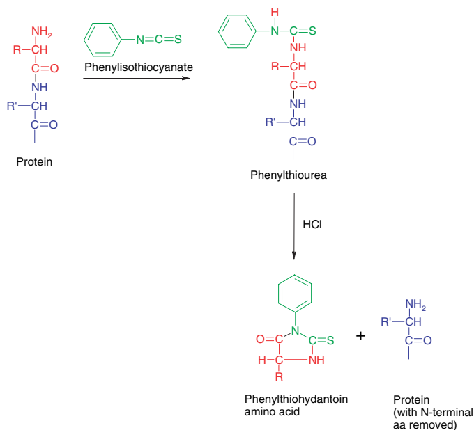
Figure 4.1. Edman-degradation of a protein. In each cycle one amino acid is cleaved off from the N-terminus and identified. The remaining protein can go directly to the next cycle.
