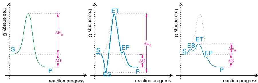
Figure 6.15. Left: A chemical reaction without a catalyst. The product has a lower free energy ( G ) than the substrate, so the reaction should proceed. However, because the substrate ( S ) first needs to be activated to a transition state ( T ) with high energy, reaction rate is slow. Catalysts accelerate the reaction rate by lowering the activation energy ( \Delta E_a ). Because they do not influence \Delta G , they also have no influence on the equilibrium position. Middle: If the substrate binding site in the enzyme were complementary to the substrate ( lock-and-key model ), enzymes would stabilise the substrate and increase the activation energy for the reaction. The reaction rate would be lowered. Right: If the binding site is complementary to the transition state ( induced fit model ) a small amount of activation energy is required to form the initial ES complex, but the binding energy ( \Delta E_b ) between enzyme and transition state mostly compensates for the activation energy required for the formation of the transition state. The change in free energy resulting from the conversion of the transition state into product then drives the formation of the EP complex, breaking the E-T bonds in the process. A further small amount of activation energy is then required to release the product from the enzyme.
